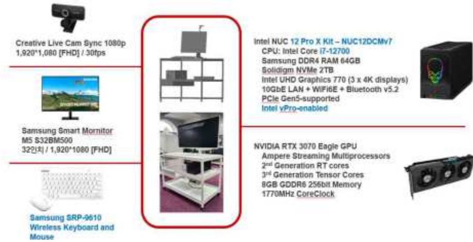
[MobileX Station 구성도]
